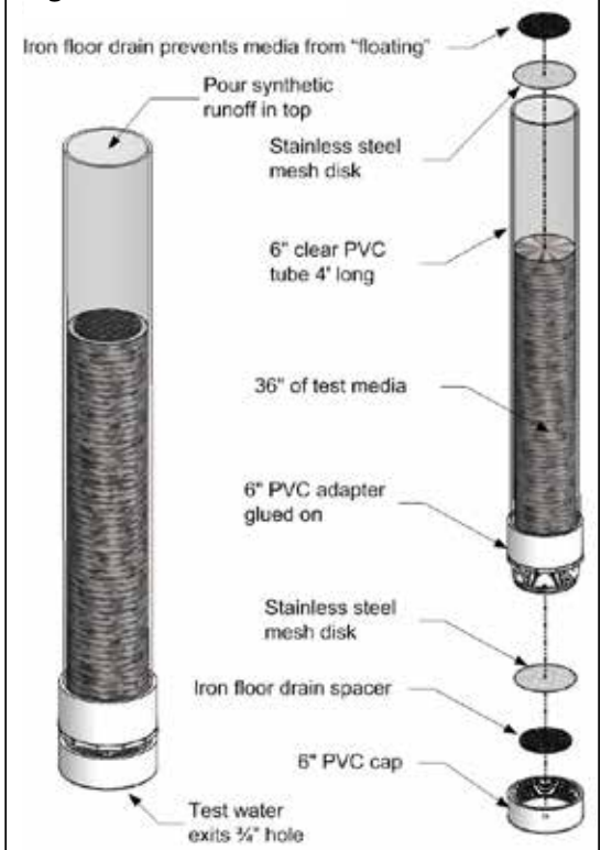
Figure 1. Test Column
